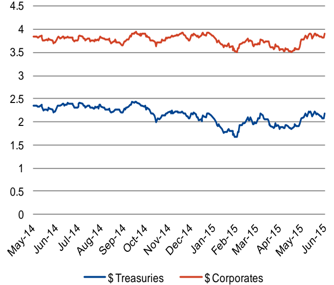
Figure 20: $ Yield
