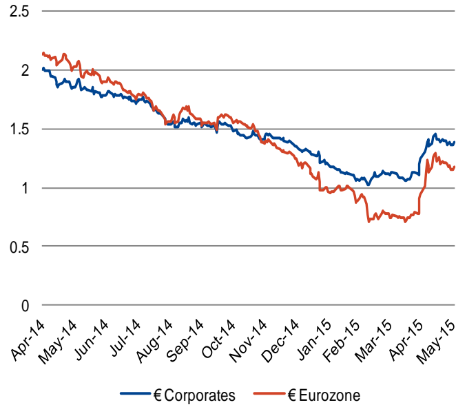
Figure 4: € Yield
