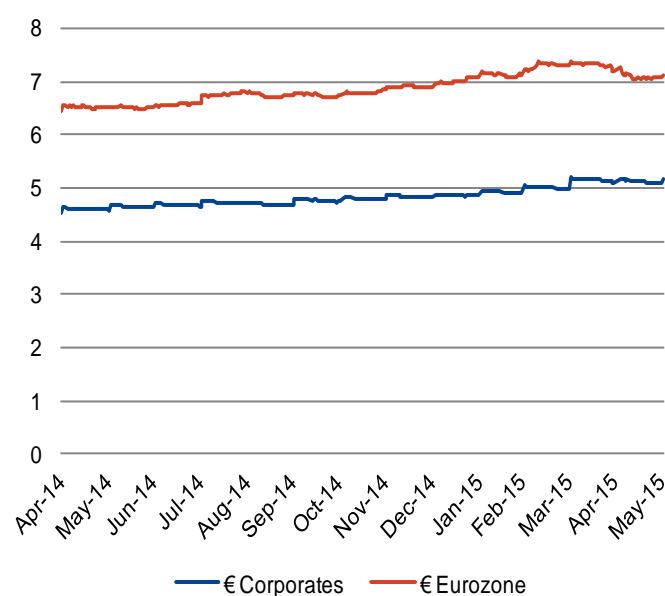
Figure 5: € Duration
