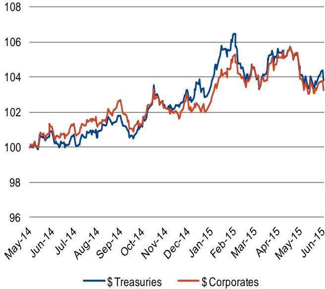
Figure 19: $ Total return
