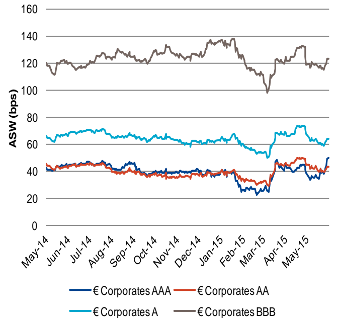
Figure 6: € ASW
