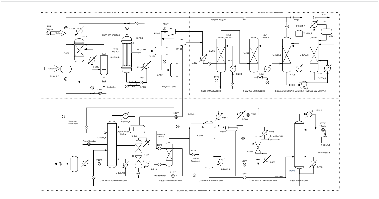
Typical Vapor Phase Process sections
